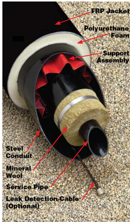
MULTI-THERM 500
