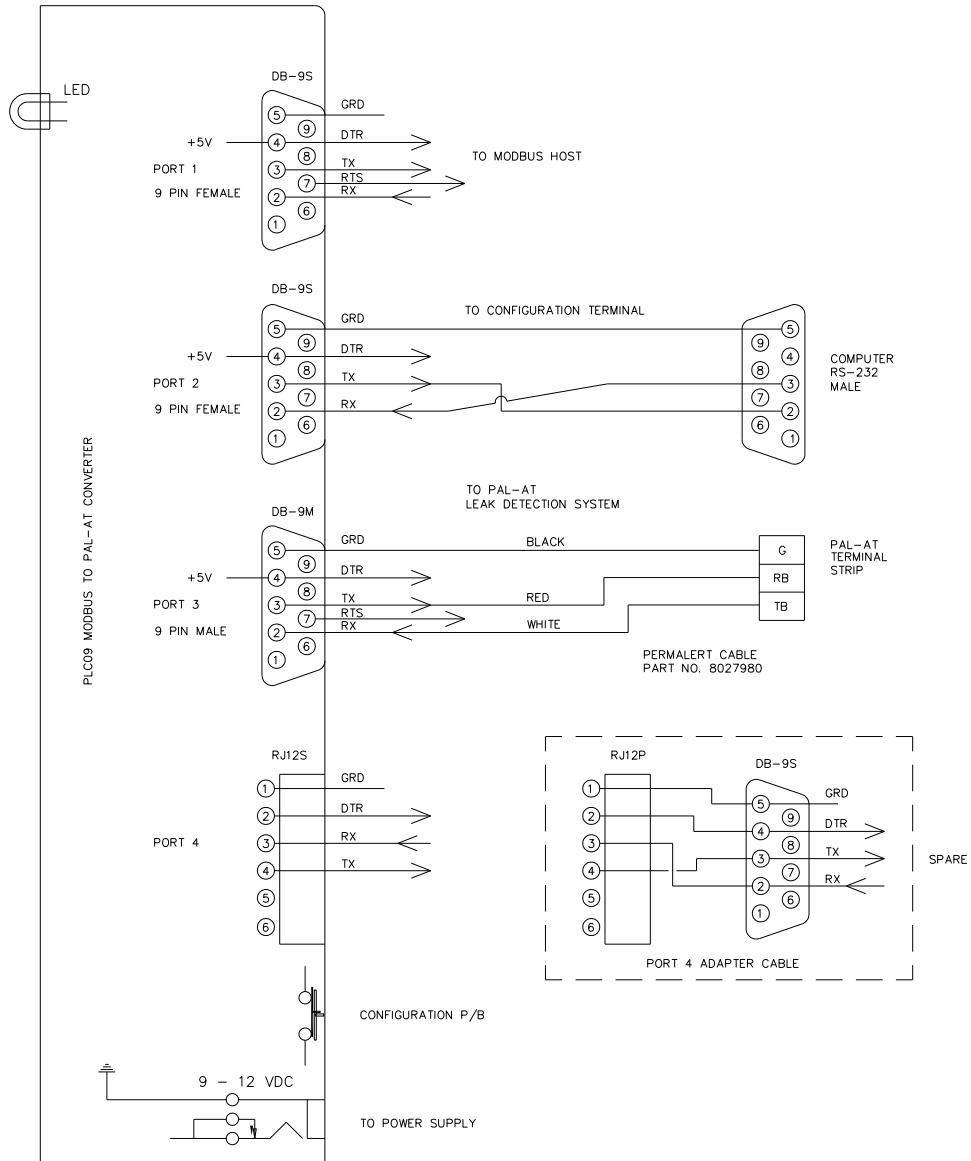
Figure 1 PAL-AT To PLC09 Connection Diagram
